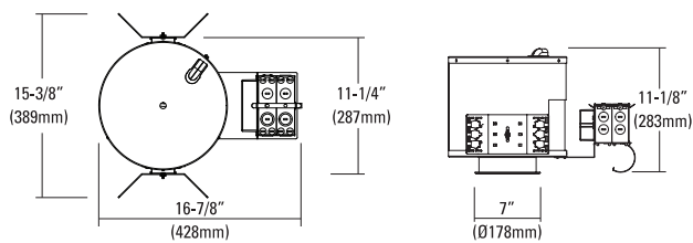
Ceiling Cut-out : Ø6-1/2" (Ø165mm)
